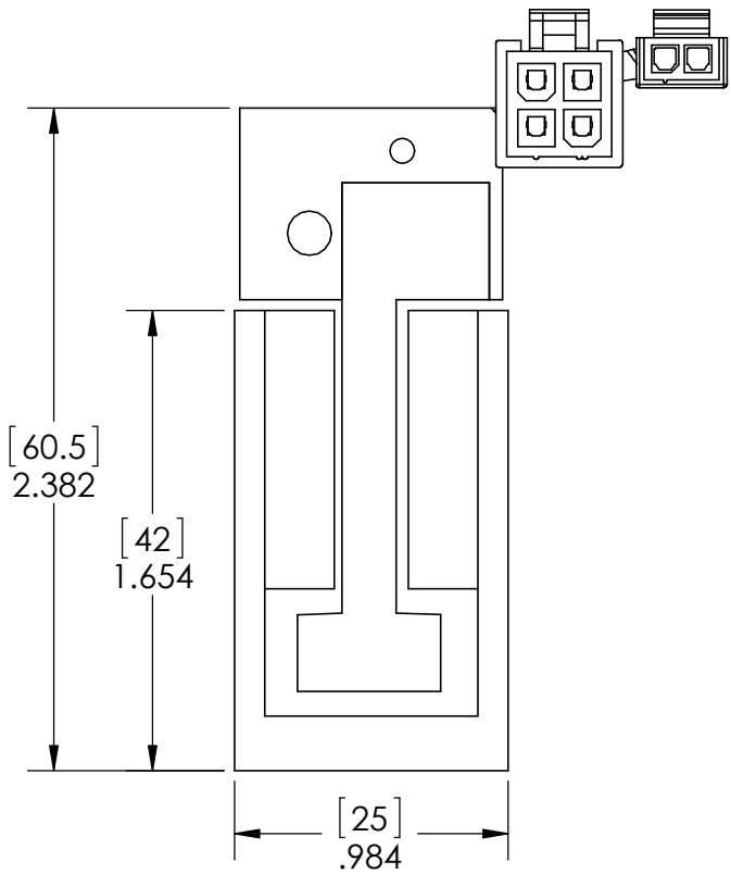
MOTOR COIL SHOWN WITH MAGNET TRACK (P/N: BLDT-B29)
